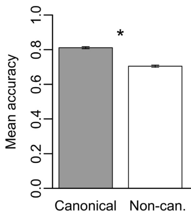
Fig. 2. Mean identification accuracy of two-word phrases containing an assimilation-licensing context by participants in Experiments 1 and 2. Results are divided by pronunciation, either Canonical or Non-canonical, as identified by three phonetically trained classifiers.
