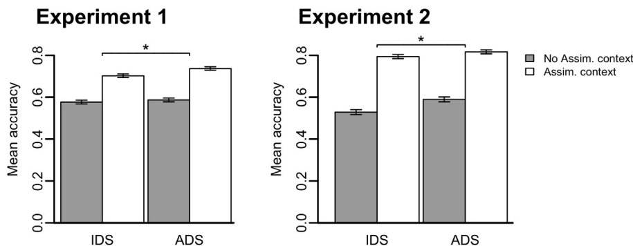
Fig. 1. Mean identification accuracy of phrases spoken in infant-directed speech (IDS) and adult-directed speech (ADS) in Experiments 1 and 2. Targets were potentially ambiguous two-word phrases that did or did not license place assimilation (e.g. cat box and cap box ), presented in isolation (Experiment 1) or whole sentences (Experiment 2). In both experiments adult listeners were more accurate in identifying the intended target in ADS than IDS.
