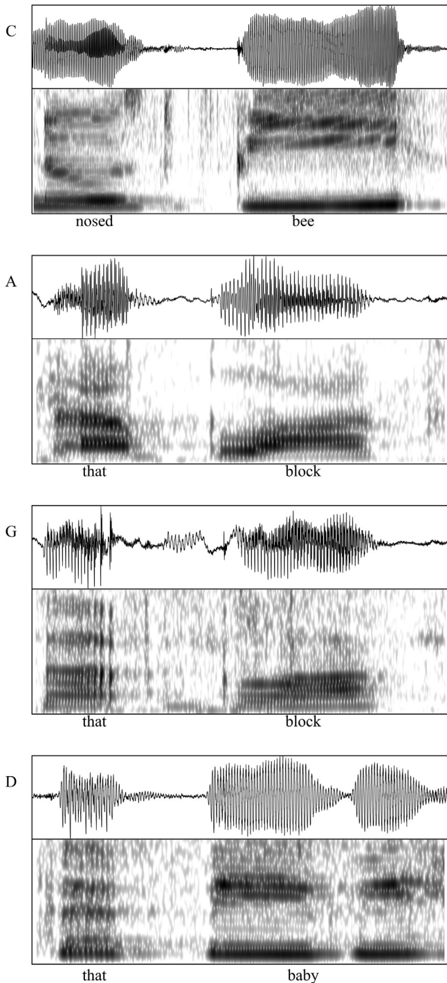
Fig. 4. Example waveforms and spectrograms of the four classification types used to analyse the corpus of spontaneous speech. The categories are Canonical (C), Assimilated (A), Glottalized (G), and Deleted (D).
