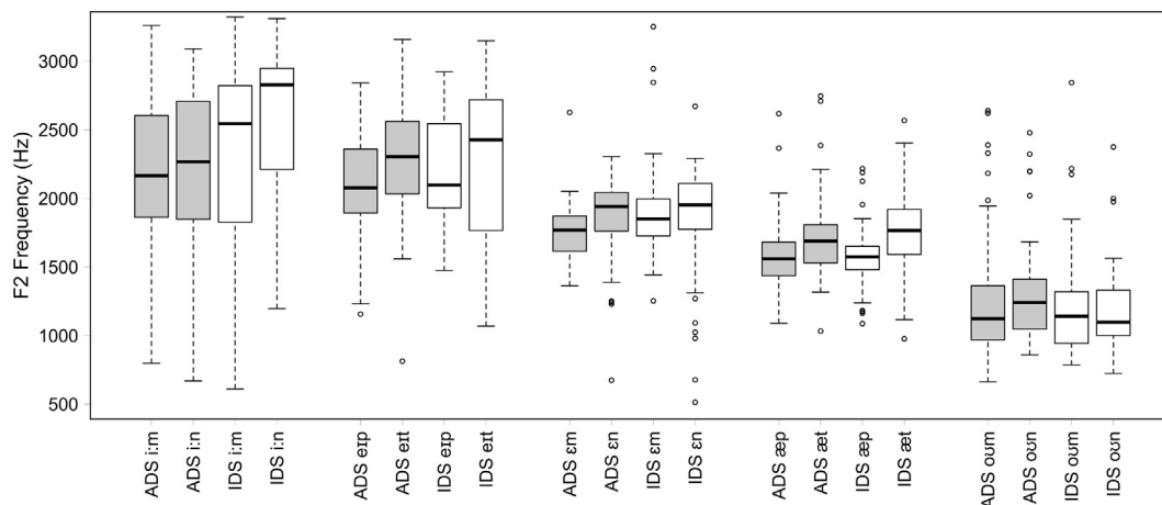
Fig. 3. Frequency of second formant at the end of the vowel in the first word of the two-word phrase. Data are grouped by vowel, and divided by Addressee (IDS or ADS) and whether the context licenses assimilation (e.g. cat box ) or not (e.g. cap box ). An ANOVA analysis of the data by vowel including the factors Addressee, Licensing Context and their interaction, revealed a significant main effect of Licensing Context ( F(1,4) = 9.75 , p = .04 ) with higher F2 frequency in a context that licenses assimilation. There was no significant effect of Addressee ( F(1,4) = 1.52 , p = .28 ), and no interaction of the two factors ( F(1,4) = 0.01 , p = .92 ).
